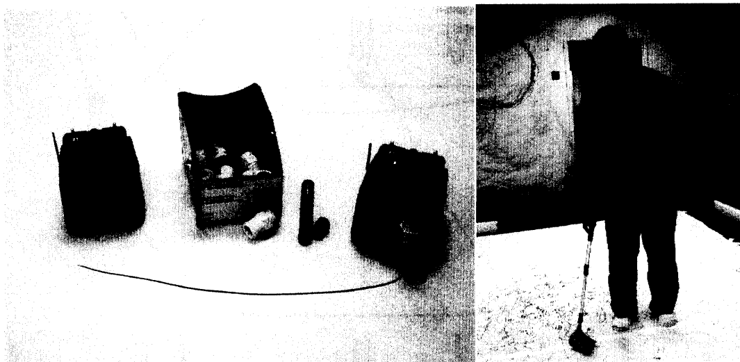
Figure 21: The state-of-the-art data collection hardware shown above used to measure path lengths on the swarm. Left: Each robot was instrumented with a magic marker. Right: The author measuring the path of a robot. (He is in a much better mood now)
