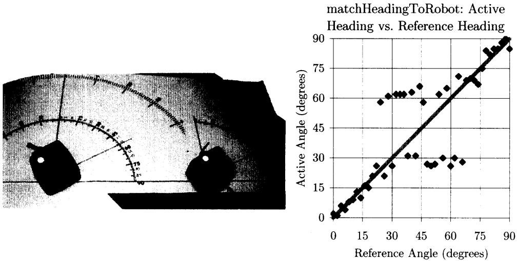
Figure 26: Left: The angleometer is used again to collect data on the matchHeadingToRobot behavior. The reference robot has its red light flashing, and the active robot has its green light on. Both reference and active robots have wire indicators. The reference robot is manually rotated to the input angle, which is selected at random to avoid having the active robot rotate in only one direction. Right: The matchHeadingToRobot behavior works well when ISIS works well, but fails when ISIS fails. Average error is 11.1^\circ , with a deviation of 12.1^\circ around the mean. Accuracy over the full 360^\circ range is 97%.
