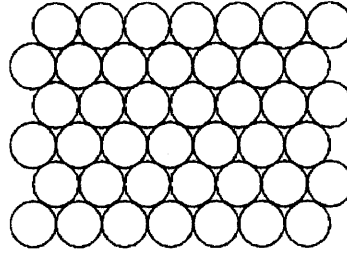
hexagonal packing
