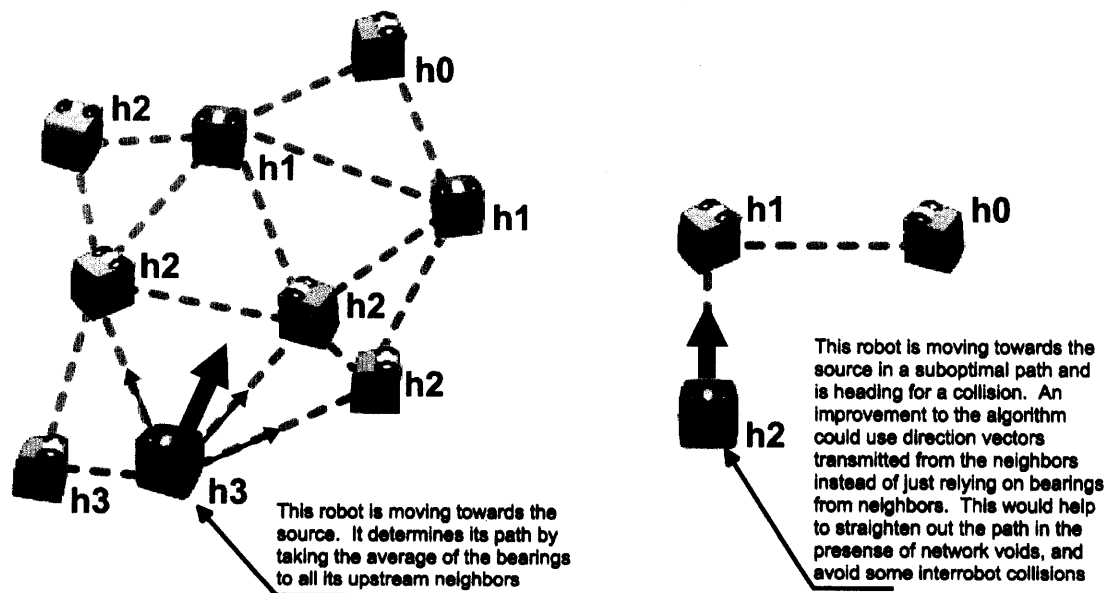
Figure 51: The navigateGradient behavior guides the active robot to the source of a gradient.
