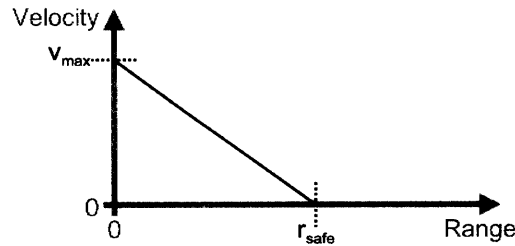
Figure 42: The disperseUniformly velocity equations command a velocity of v max when the active robot is close to a neighboring reference robot. The commanded velocity falls to zero when the active robot is further than r safe from the reference robot..
