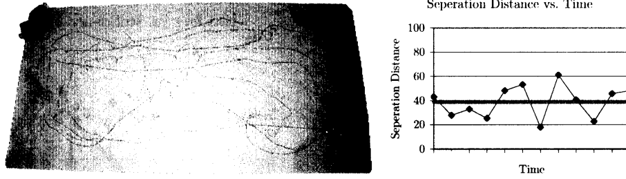
Figure 27: Left: The followRobot behavior produces the traces above. The red robot is the leader, and the green the follower. Each robot is programmed to “twitch” every two seconds so that their separation distances can be compared from the traces. Right: The commanded distance is 40 cm, and the average measured inter-robot separation is 39 cm, which yields a accuracy of 97% and a path efficiency of 114%. Both of these metrics were distorted somewhat because turns allow the follower to take “shortcuts” and round the corners on a shorter path than the leader.
