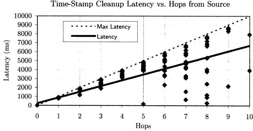
Figure 19: Data collected from time-stamp clean-up trials on a 39-robot swarm. The max latency line indicates the threshold between valid time-stamps and discard timestamps. In the swarm, p is 4 and t_n is 250 ms, which gives us a clean-up rate of 1 second/ hop. The clustering of data points underneath the max latency line shows how robots further away from the source remove their messages only after their parents have done so. The data in the lower right most likely is from network errors that cause those robots to lose their gradient message and record a spurious clean-up time.
