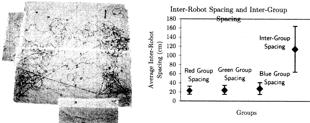
Figure 61: Left: These traces show the results of the clusterIntoGroups behavior. Right: The graph shows group spacing and inter-group spacing.
