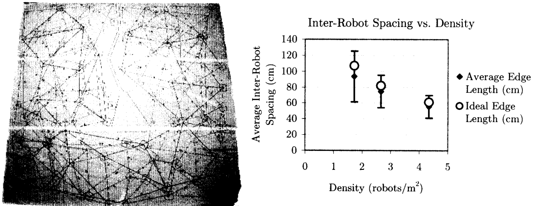
Figure 45: These traces show some results of the diprseUniformly behavior. After dispersing, the average inter-robot separation was 90% of the theoretical optimum. The path efficiency of this algorithm is low, as the robots are in constant motion, and was no higher than 6%.
