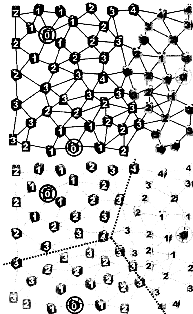
Figure 9: The normal gradient compare function will tessellate the swarm into Voronoi cells based on the number of hops each robot is from the source. This can be a convenient way to divide the robots into groups.
