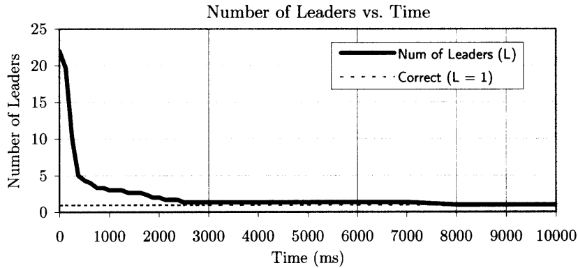
Figure 13: Gradients with lateral inhibition can be used to elect a leader among several robots. The graph above shows the number of leaders vs. time for several trials of this algorithm. It takes one propagation time for one leader to be elected and for all other robots to know it. In the data above, the leader is elected in an average of 4125 ms, which is very long compared to 1575 ms predicted by the data in Figure 11. This network was denser and had several turns, so packet collisions and bad links could have contributed to this error.
