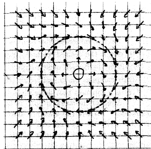
Figure 31: This is a sketch of the orbitRobot vector field. This vector field is the sum of the velocity outputs of orientForOrbit + moveForward produce a velocity vector field with a stable limit cycle at a radius d from the reference robot. Robots that move along this field will orbit the reference in approximately a circular path..
