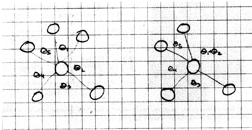
Figure 62: Robots use the bearing differences between each of their neighbors to determine whether or not they are on the edge of the network. Left: The separation angle \theta_2 is the largest, but is insufficient to declare this robot to be on the edge. Right: With one neighbor removed, the largest angle becomes \theta_1 + \theta_2 . This angle is large enough to declare the active robot to be an edge.
