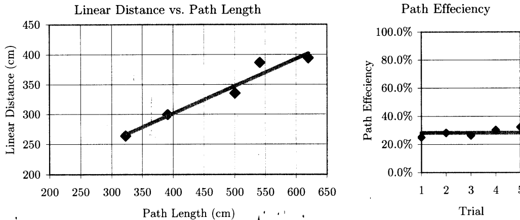
Figure 52: The navigategradient behavior shown a tight correlation between linear distance and path length. Average path efficiency is 28%
