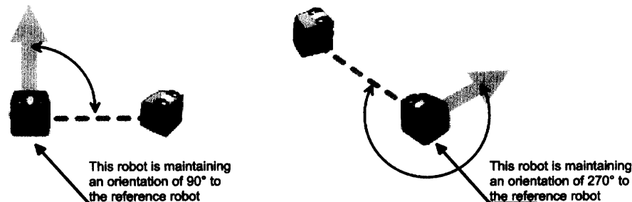
Figure 22: The orientToRobot behavior is a flexible way to orient an active robot with respect to a reference robot. The active robot rotates to the desired orientation relative to the reference.
