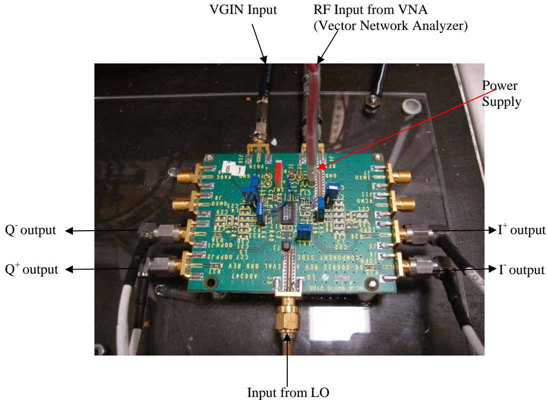
Figure 33 AD 8347 Quadrature demodulator by Analog Devices.
