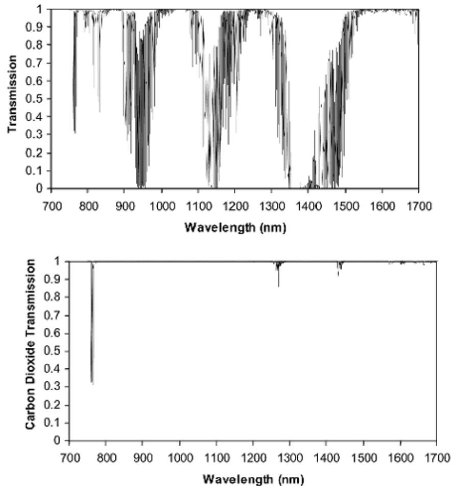
Figure 16. Absorption of Water Vapor (top) and of CO 2 (bottom) [From Ref16]
